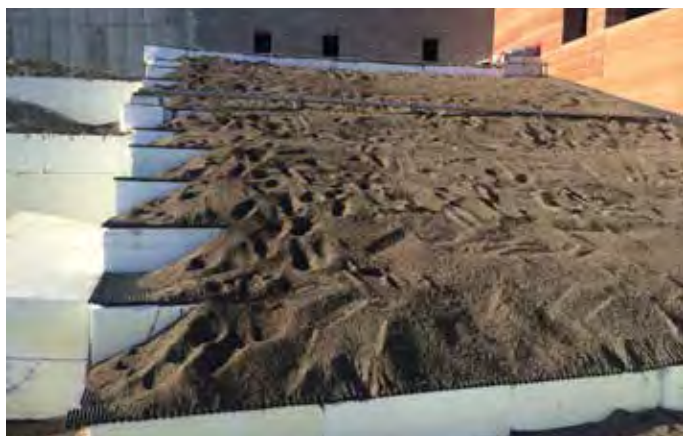
Stepped geofoam used to create topography - Brinton Museum - Brinton, WY
