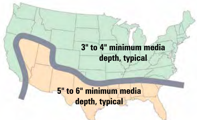
Minimum Extensive Garden Roof Assembly Media Depth
