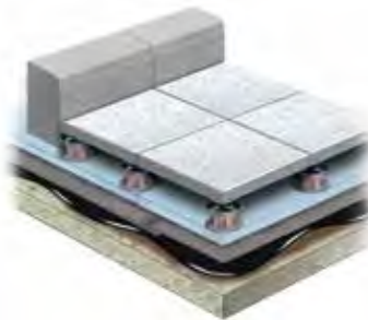
Ultimate Assembly® Architectural Pavers and RockCurb
