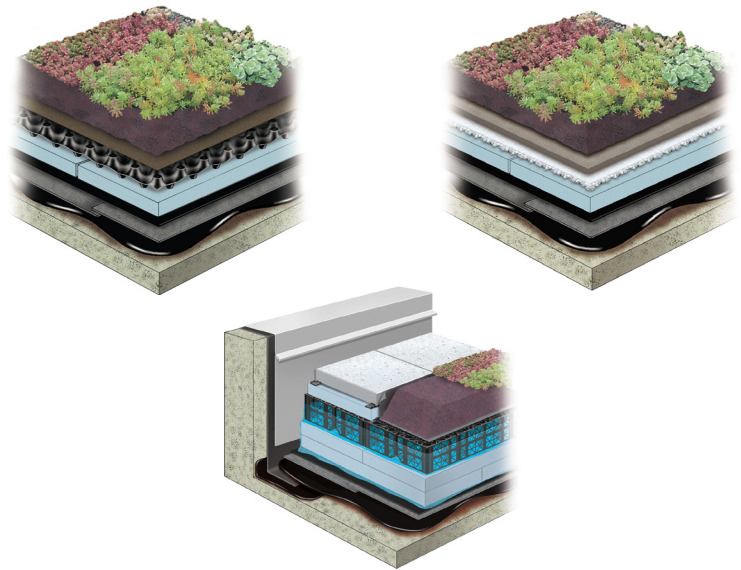
Typical stormwater management assemblies
