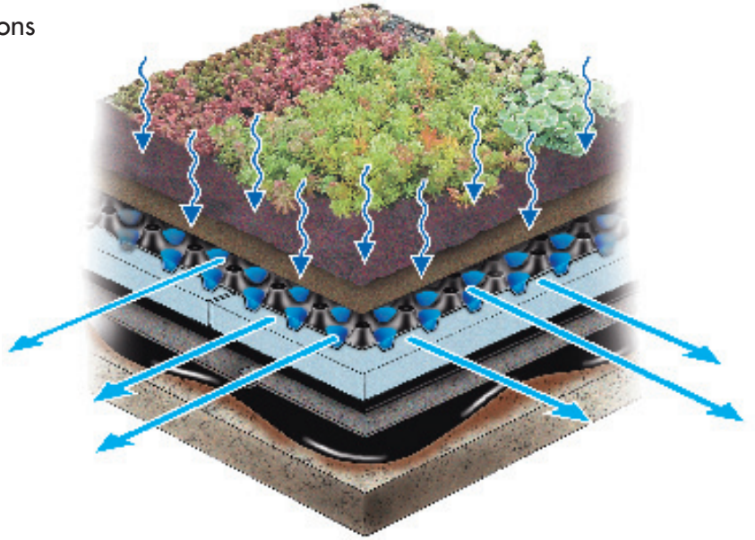
Typical garden roof assembly
